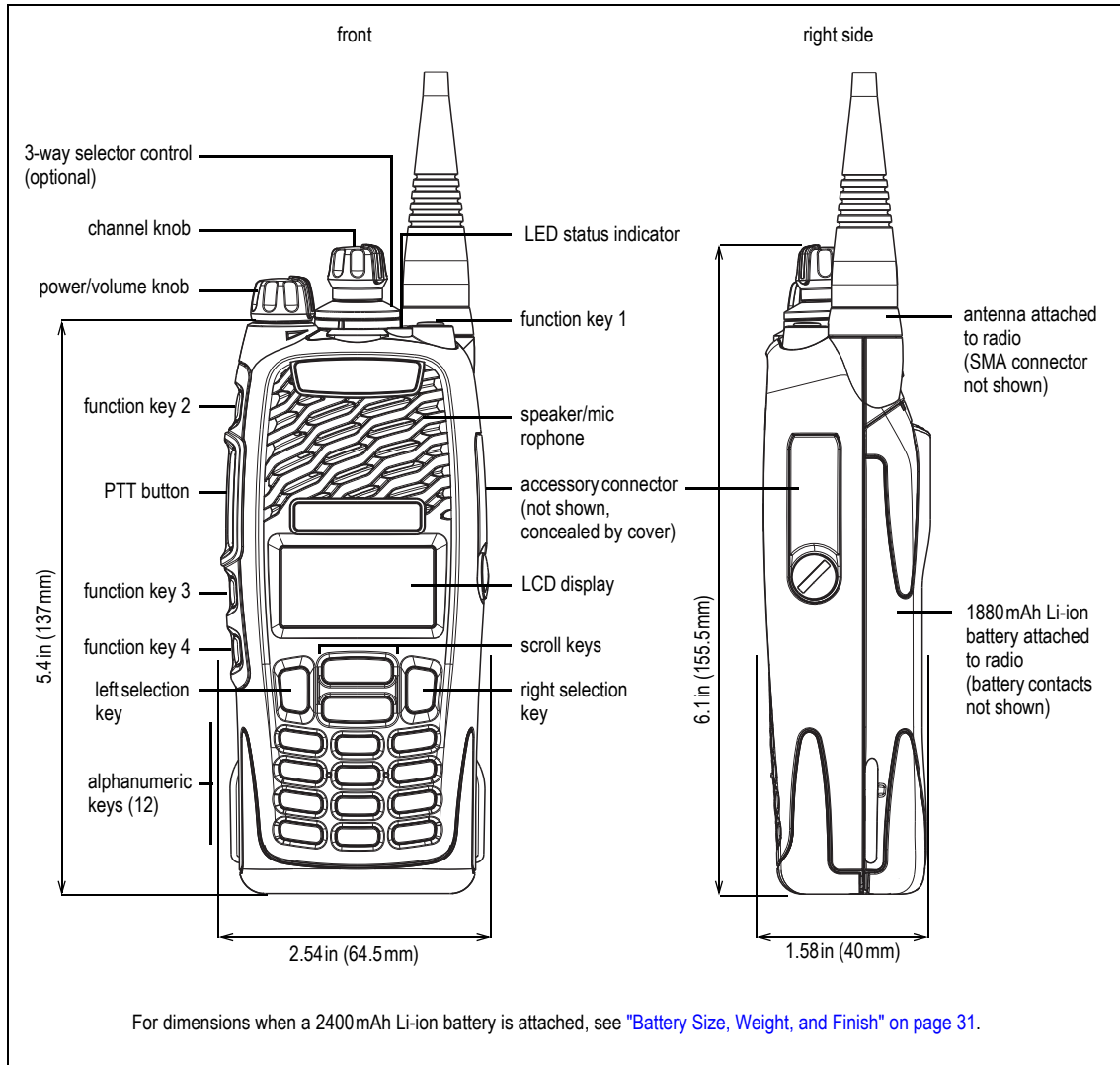
Figure 4.1 TP9300 (16-key radio) dimensions and user interface
